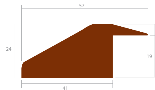
Reducer
